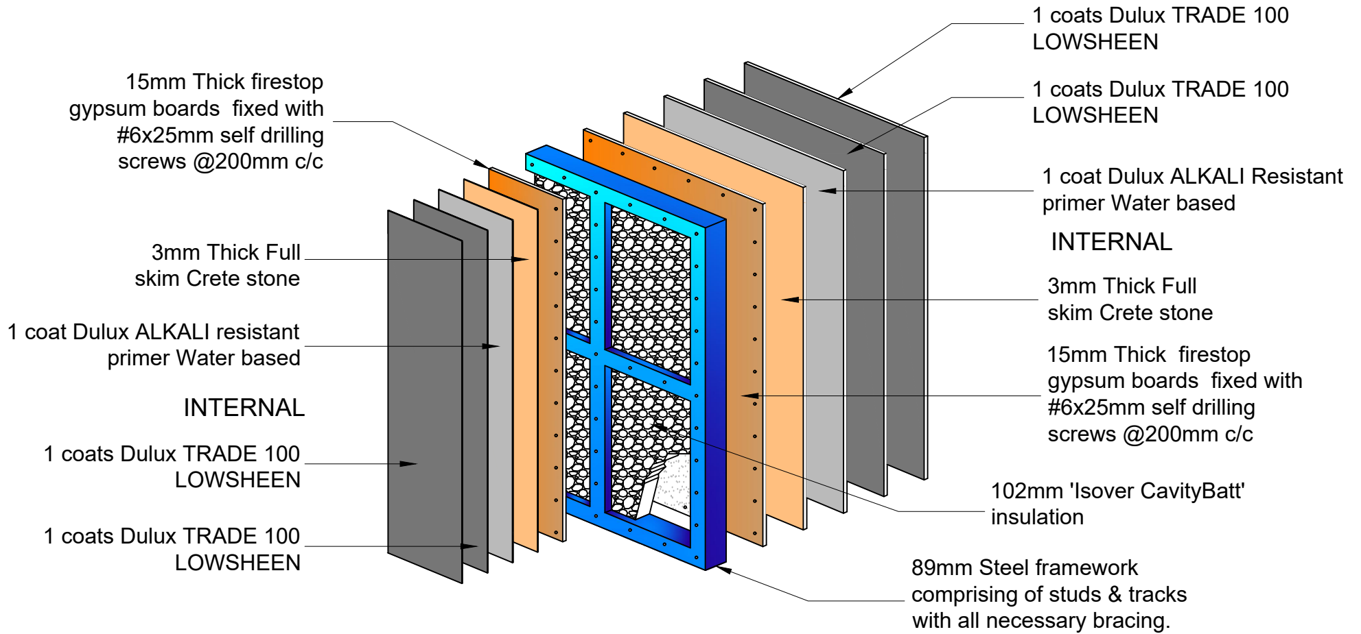
Internal LFS Wall Detail - 1 Hour Fire Rating
