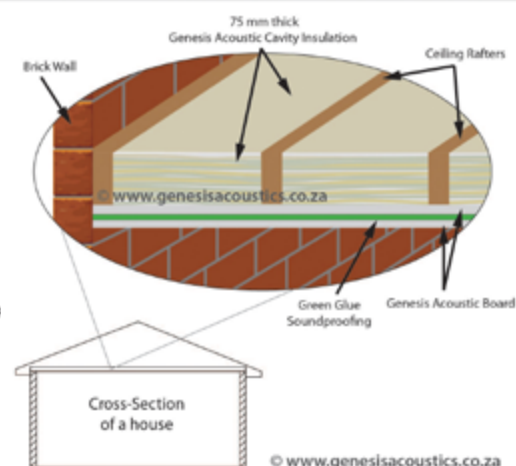
SOUNDPROOFING A SIMPLE CEILING
