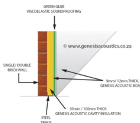
SOUNDPROOFING A BRICK WALL
